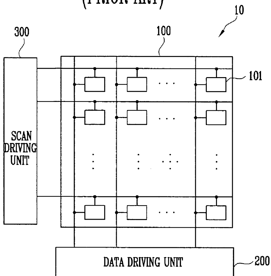
FIG. 2 (PRIOR ART)
